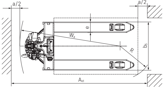
ECH 12C/15C vista superior
